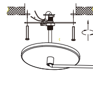
Electricity Module and Cover Plate (Driver not included) ETMSC01-BK, -WT 5"L x 5"W x 0.25"H
