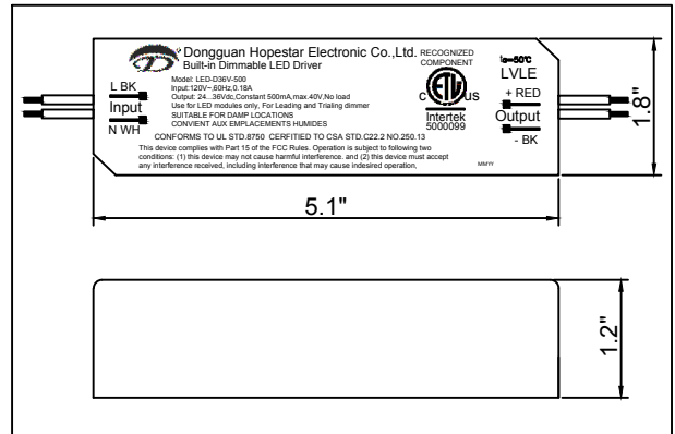
LED Driver Diagram
