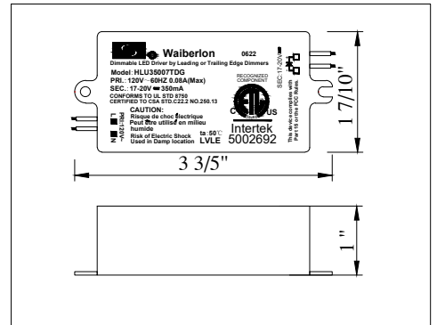
LED DRIVER DIAGRAM
