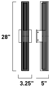
E30318-BK Outdoor Wall
