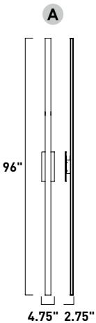
E42348-ABZ, -BK, -SA, -WT Outdoor Wall
