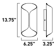
E30152-BKGLD, -SAWT Outdoor Wall
