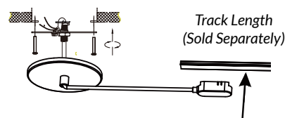
Electricity Module and Cover Plate (Driver not included) ETMSC01-BK, -WT 5"L x 5"W x 0.25"H
