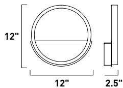
E24320-BKGLD, -WTGLD Wall Mount
