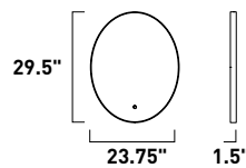
E42012-90AL, -90BRZ Mirror
