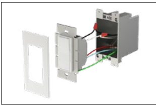
Dimmable Driver & Switch SWT898-2460WT 60W 2.25"L x 2"W x 4.25"H
