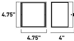
E23216-BK, -WT Outdoor Wall
