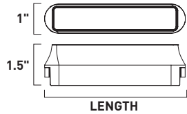
100° Standard lens
